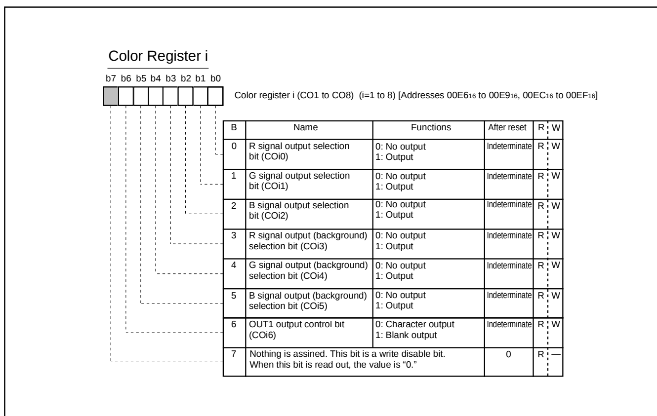
Fig. 8.10.19 Color register i (i = 1 to 8)
