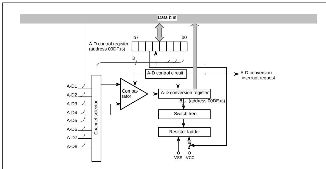
Fig. 8.8.1 A-D Converter Block Diagram
