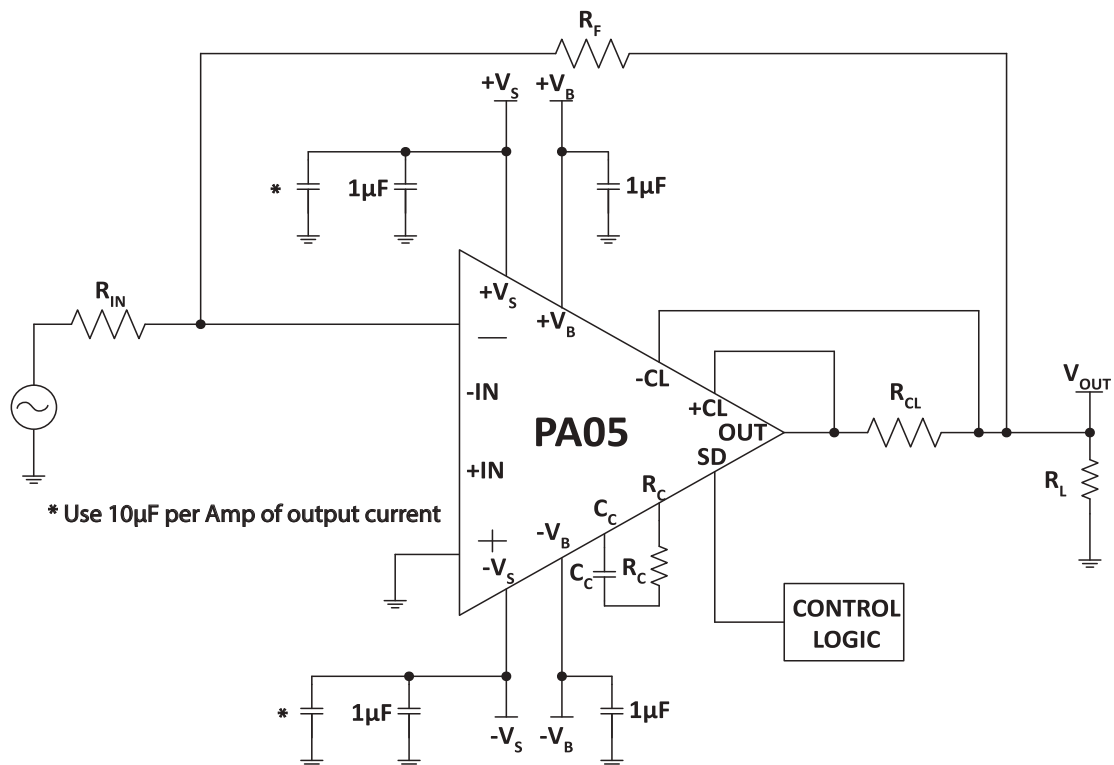
Figure 2: Typical Connections
