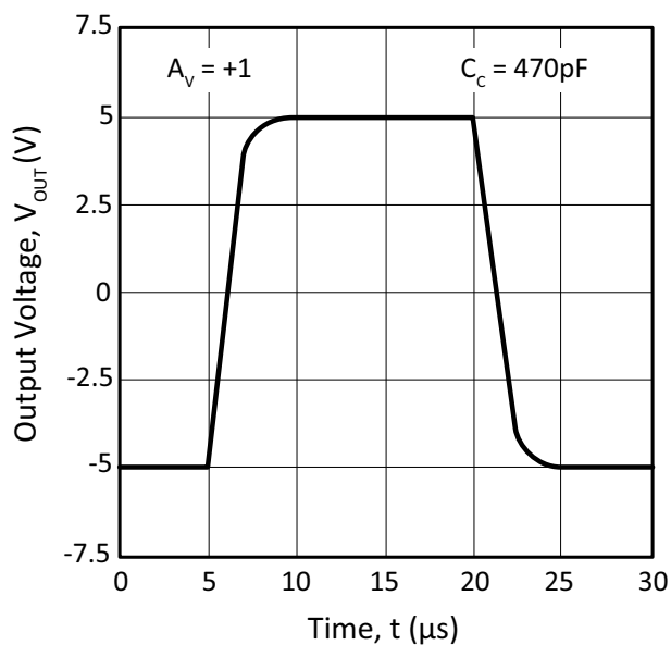
Figure 11: Pulse Response
