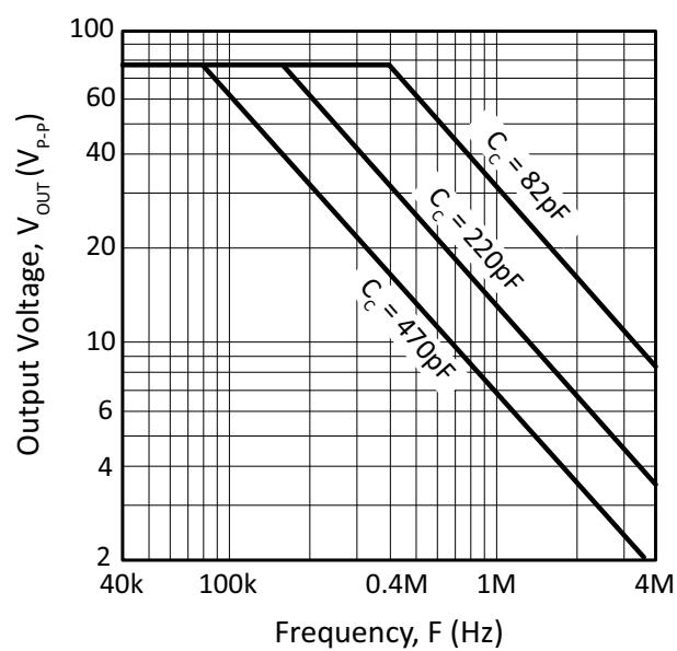
Figure 15: Power Response
