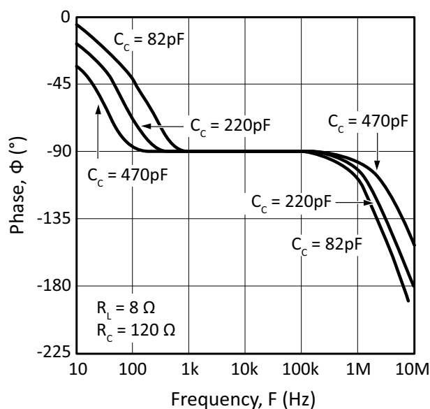
Figure 7: Phase Response
