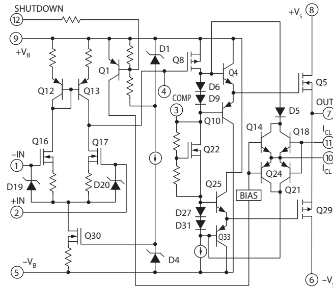
Figure 1: Equivalent Schematic
