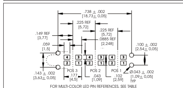
RECOMMENDED PAD LAYOUT - MULTI - COLOR
