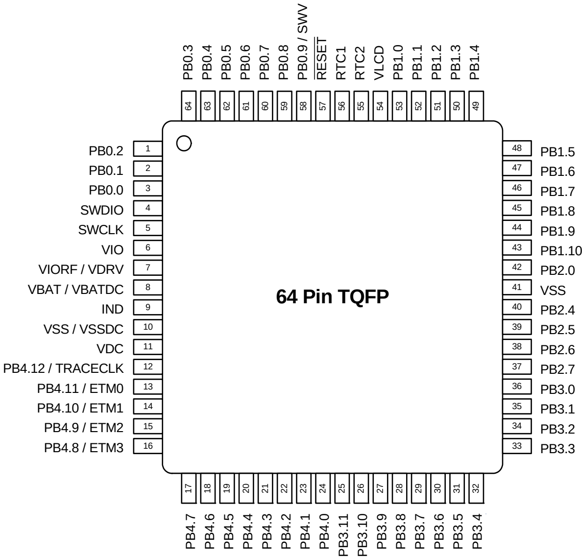
Figure 6.3. SiM3L1x6-QQ Pinout
