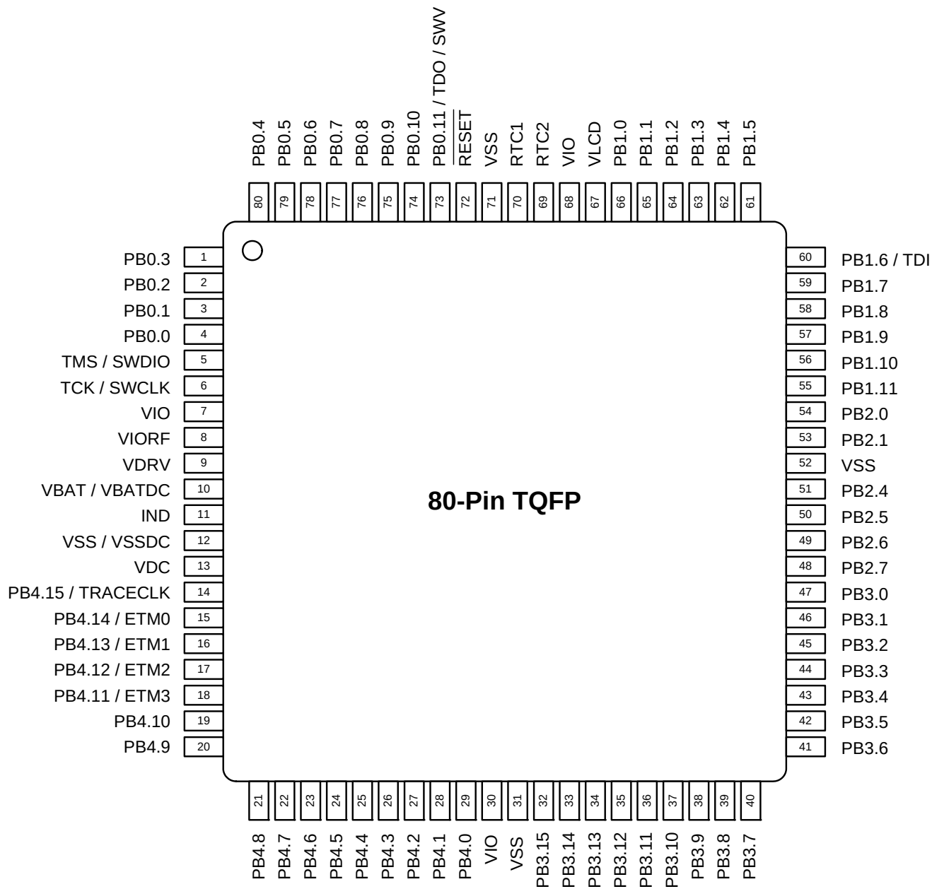
Figure 6.1. SiM3L1x7-QG Pinout
