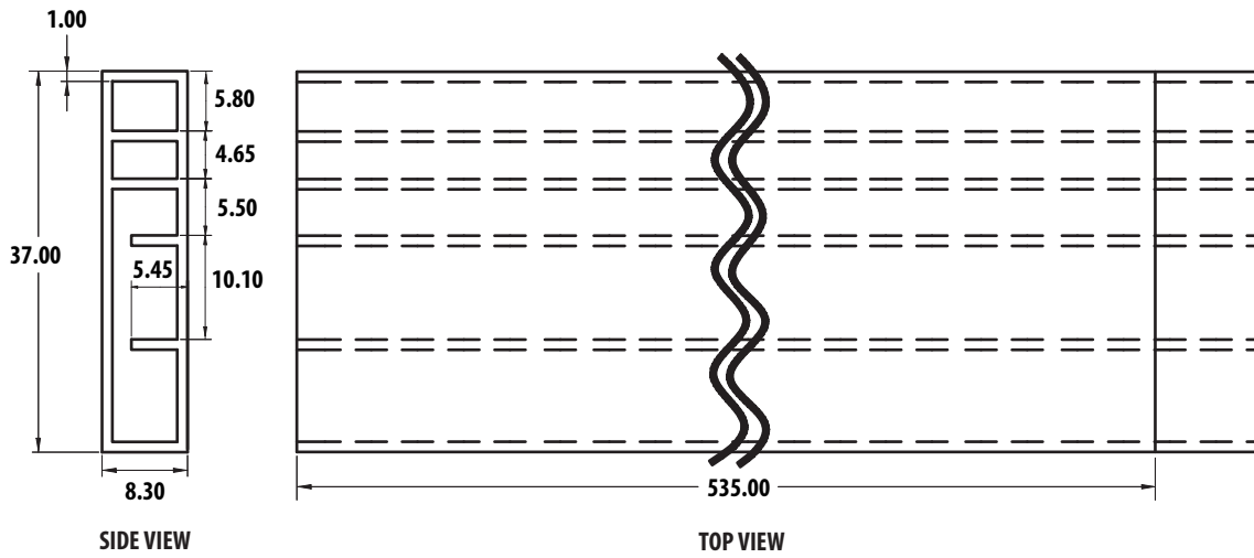
Figure 16. Tube dimensions.
