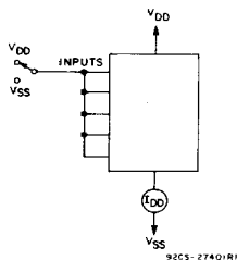
Fig. 11—Quiescent device current test circuit.
