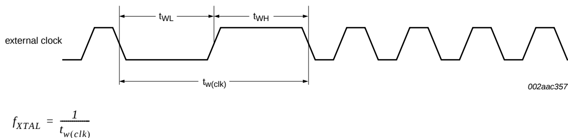
Fig 14. External clock timing
