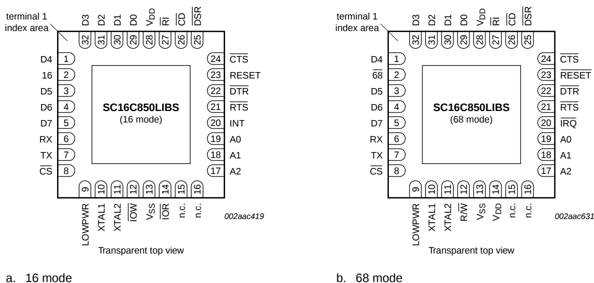
Fig 5. Pin configuration for HVQFN32
