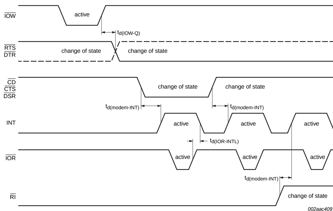
Fig 15. Modem input/output timing (16 mode)
