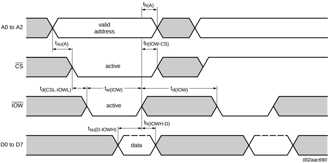
Fig 10. General write timing (16 mode)
