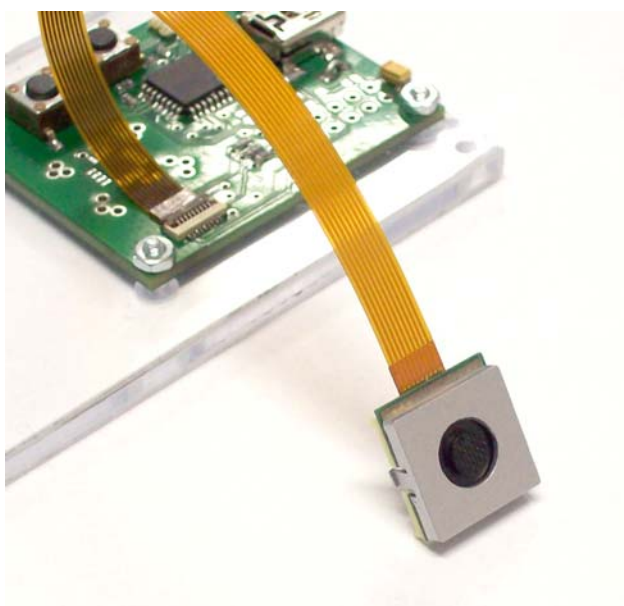
Figure 1: AS5011 pointing module
