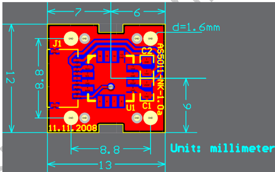
Figure 7: AS5011_NK_1.0 navigation module PCB, bottom view
