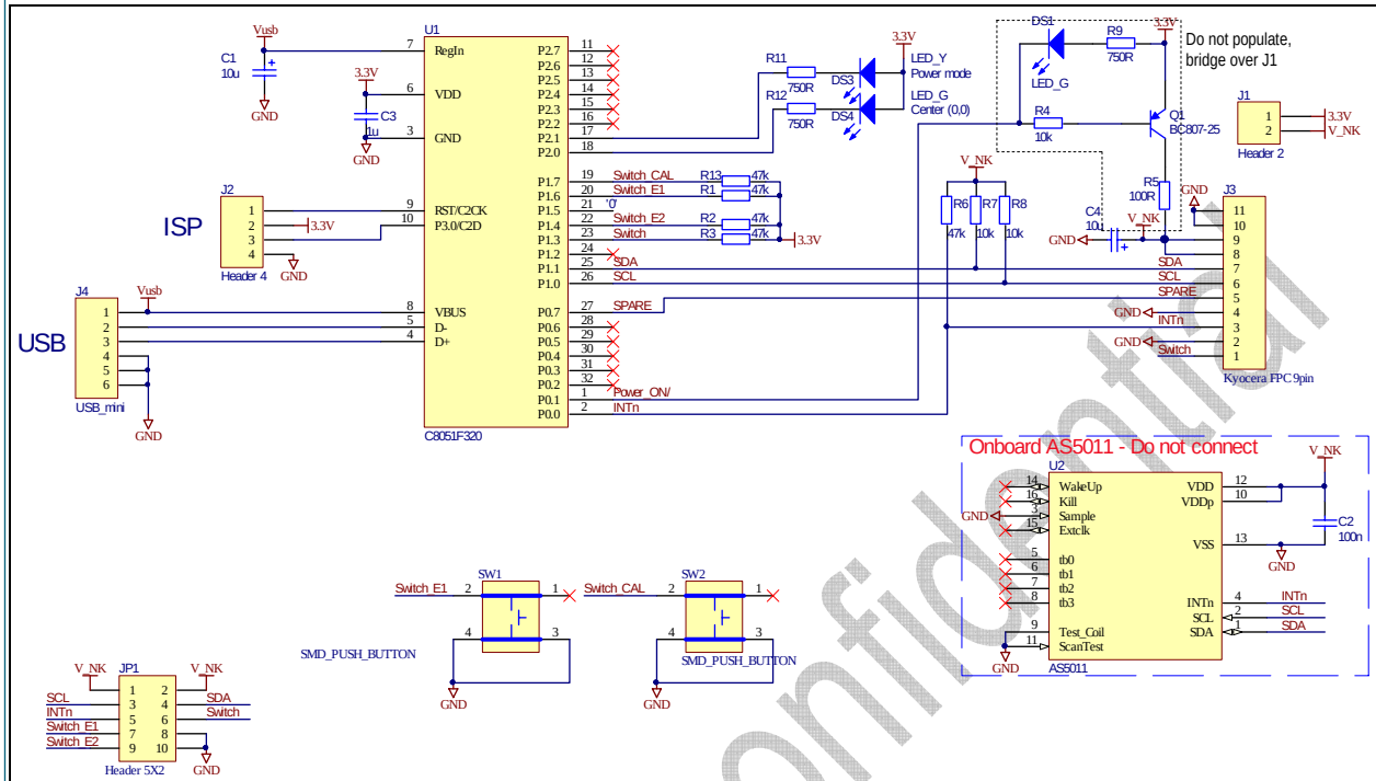
Figure 5: AS5011_NB_1.1 USB Interface schematics
