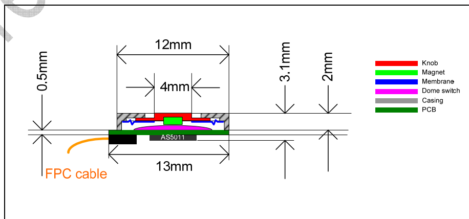
Figure 8: Module mechanics stack up
