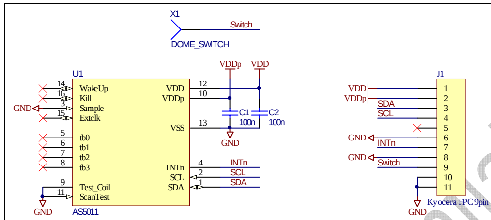
Figure 6: AS5011_NK_1.0 navigation module schematics
