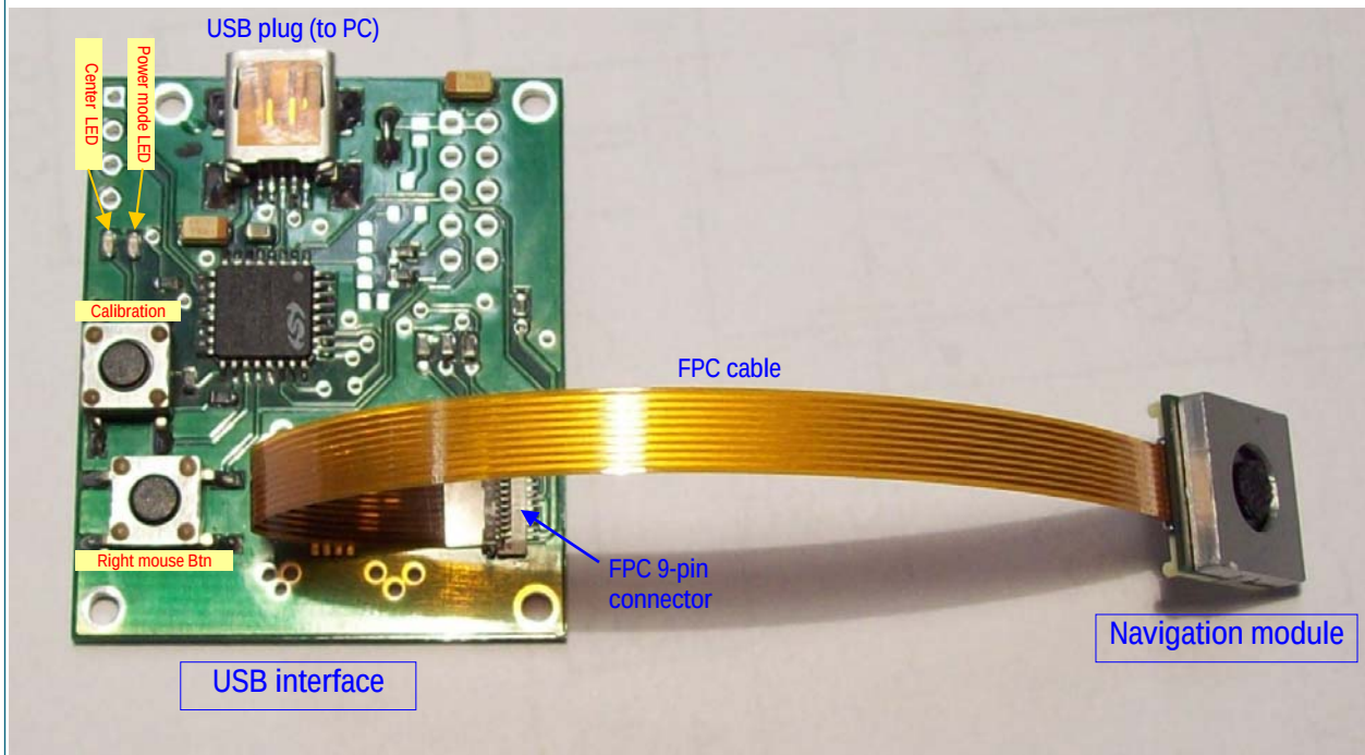
Figure 2: AS5011 demoboard
