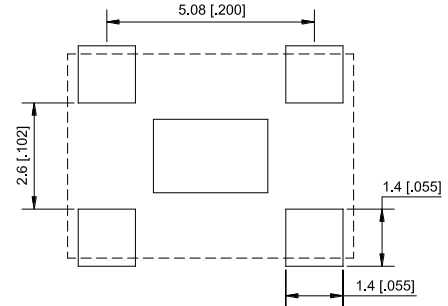
Recommended Solder Pad Layout units: mm[inch]
