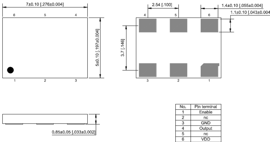
External Dimensions
