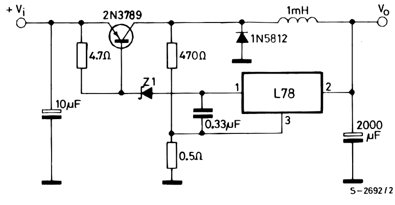
Figure 19. High input voltage circuit (configuration 1)
