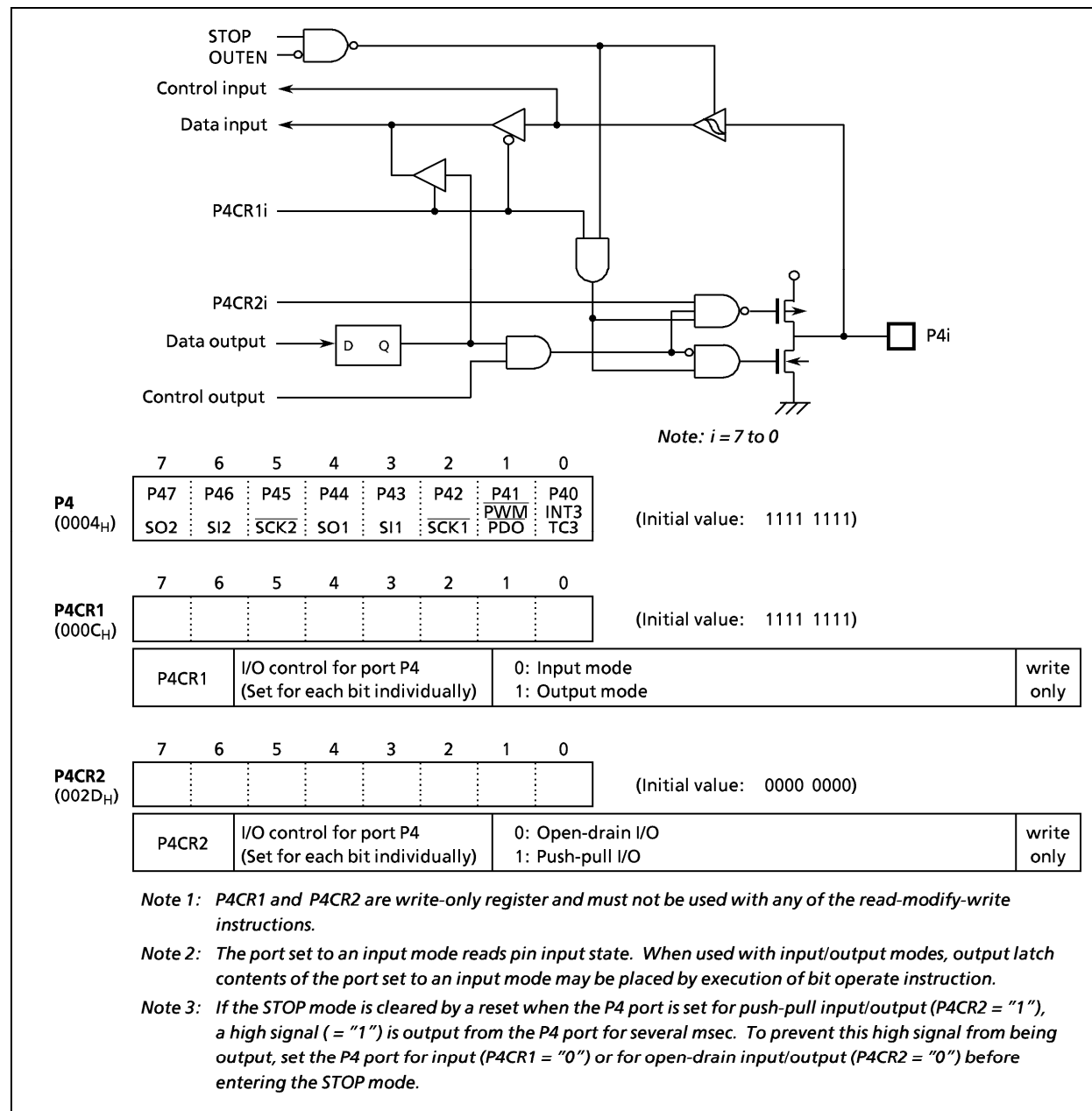
Figure 2-6. Port P4
