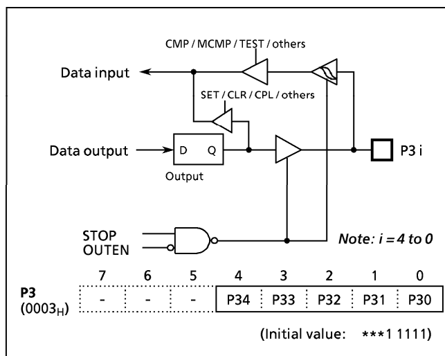
Figure 2-5. Port P3
