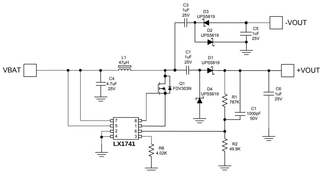
Figure 6 – Application of Dual Output, ± 20V @ 2mV
