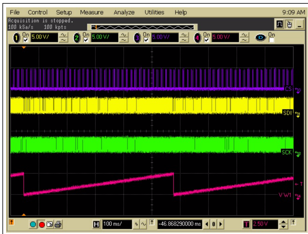
FIGURE 2-6: Screen Capture of Program 1 Output Waveforms.
