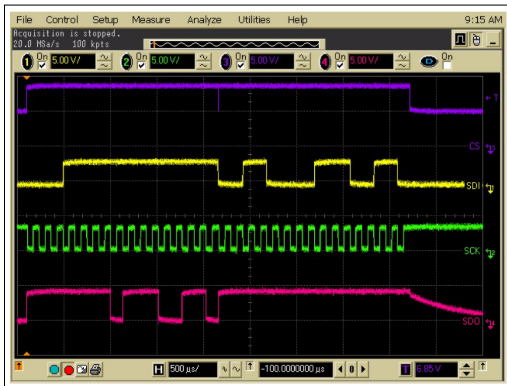
FIGURE 2-7: Screen Capture of Program 2 Non-Volatile Write Waveform.
