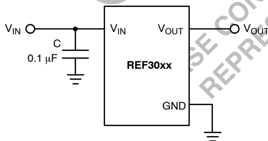
Figure 1. Application Circuit
