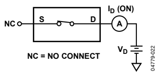
Figure 23. On Leakage
