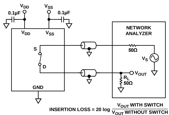
Figure 29. Bandwidth
