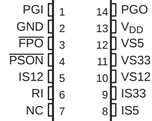
D OR N PACKAGE (TOP VIEW)
