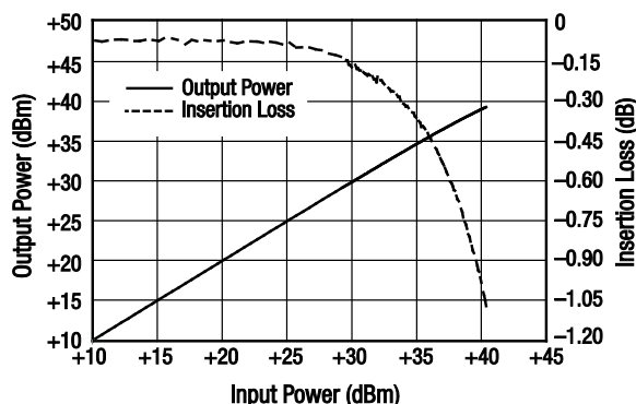
Figure 4. Output Power and Insertion Loss vs Input Power ( f = 2.0\text{ GHz} )
