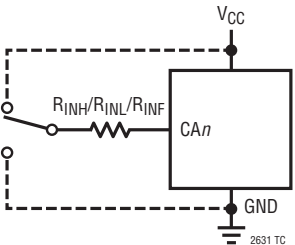
Test Circuit 2
