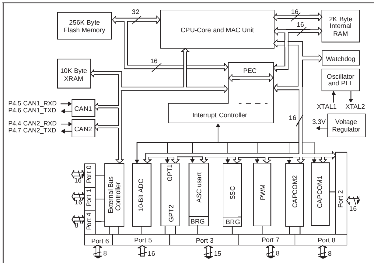
Figure 3 : Block Diagram
