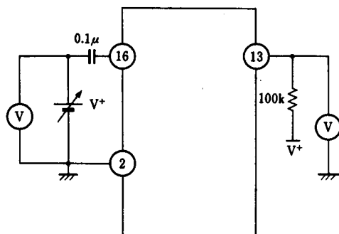
Test Circuit 3
