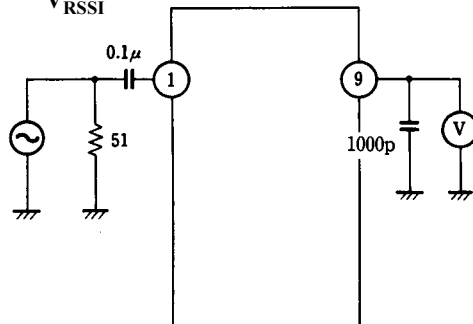
Test Circuit 10
