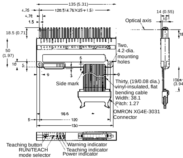
Mounting Dimensions
