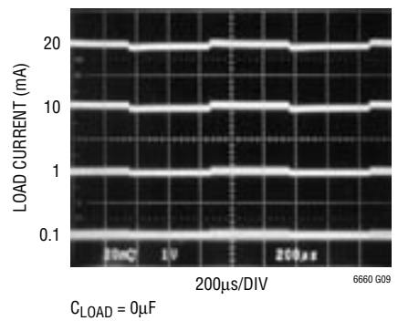
2.5V Transient Response
