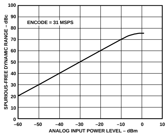
Figure 11. Two-Tone SFDR vs. Analog Input Level
