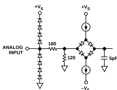
Analog Input Stage
