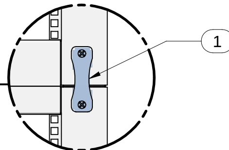
DETAIL A TYP FRONT & BACK OF CABINETS
