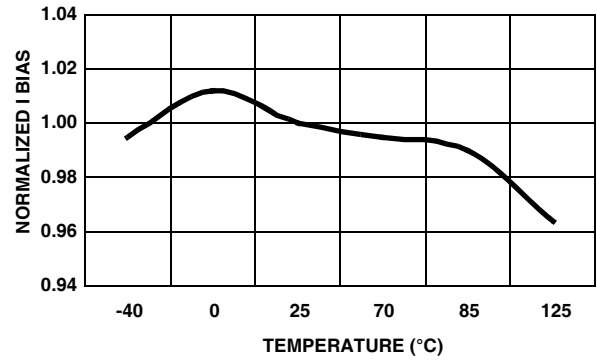
FIGURE 4. NORMALIZED I_{BIAS} ( V_{BIAS} = 3.3\text{V} ) vs TEMPERATURE
