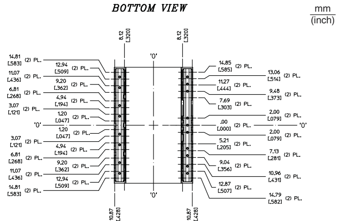
BOTTOM VIEW
