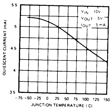
Quiescent Current
