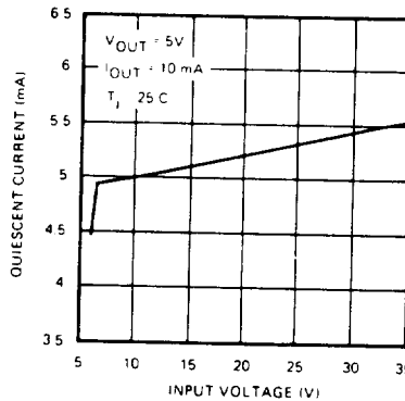
Quiescent Current
