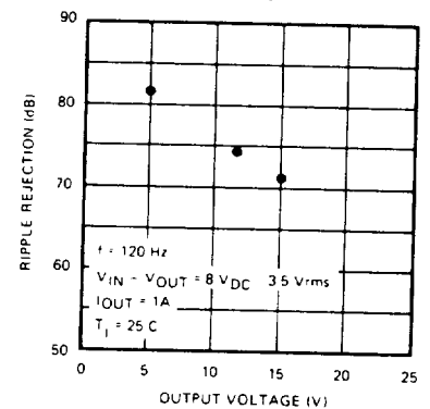
Ripple Rejection
