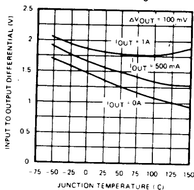
Dropout Voltage
