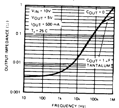
Output Impedance
