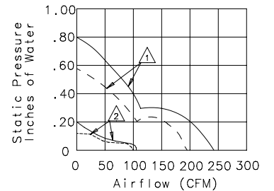
Performance Curve: 6 in. Fans
