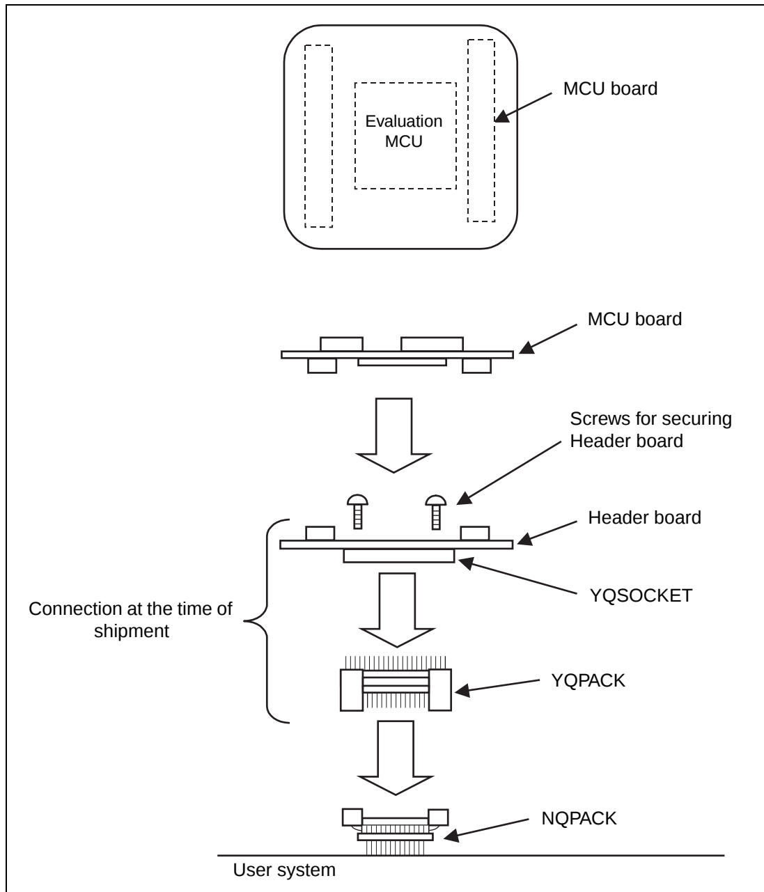
Figure 5 Connecting MCU board/header board to user system
