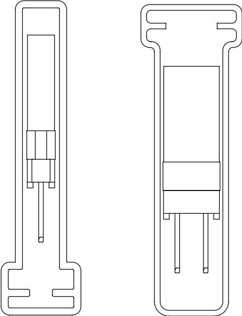
FIG 7 TUBE VIEWS
