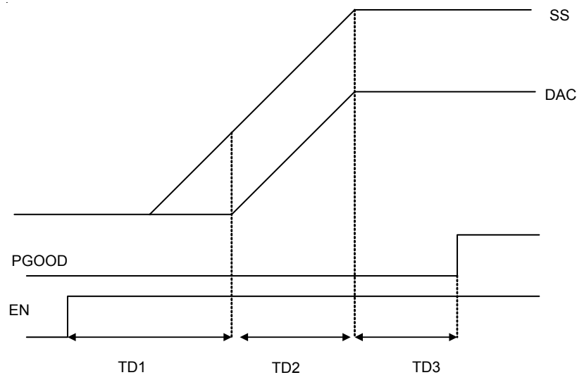
Figure 4. Soft-Start Waveform
