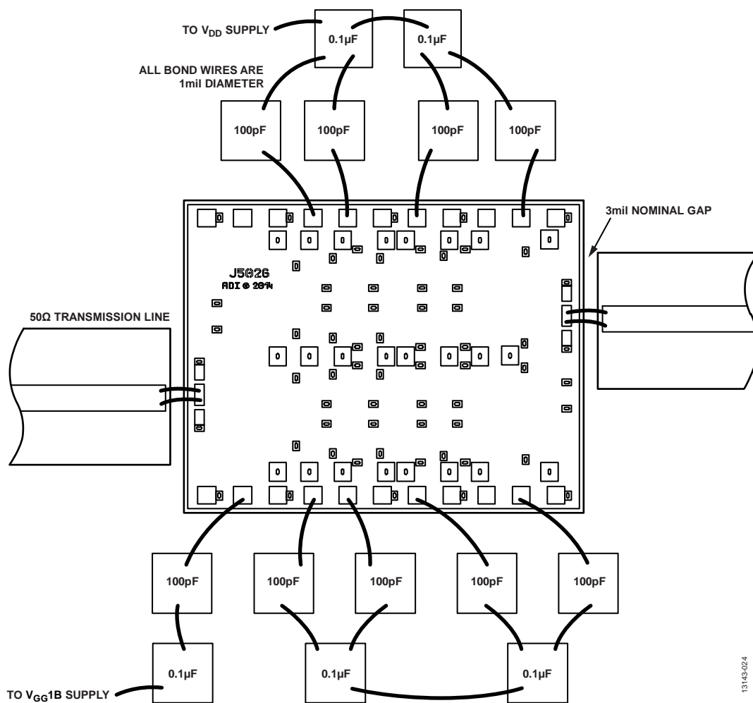
Figure 40. Assembly Diagram
