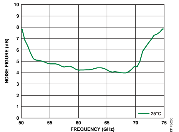
Figure 33. Noise Figure vs. Frequency at 25°C
