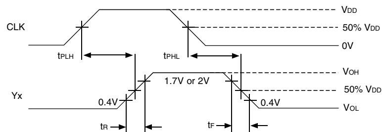
Voltage Waveforms Propagation Delay Times
