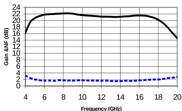
Gain & NF @Config; P1=N2=grounded
