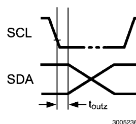
FIGURE 9. Data Output Timing
