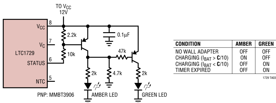
Using STATUS Pin to Indicate Charge Status
