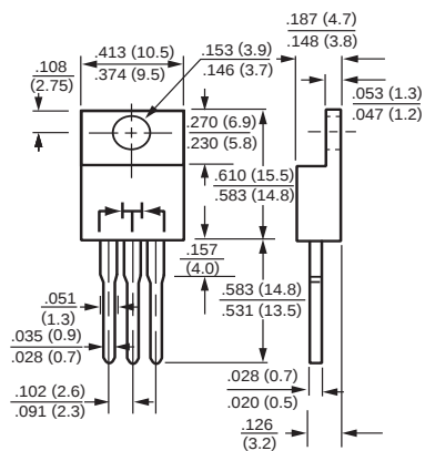
TO-220
