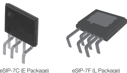
Figure 2. Package Options.
