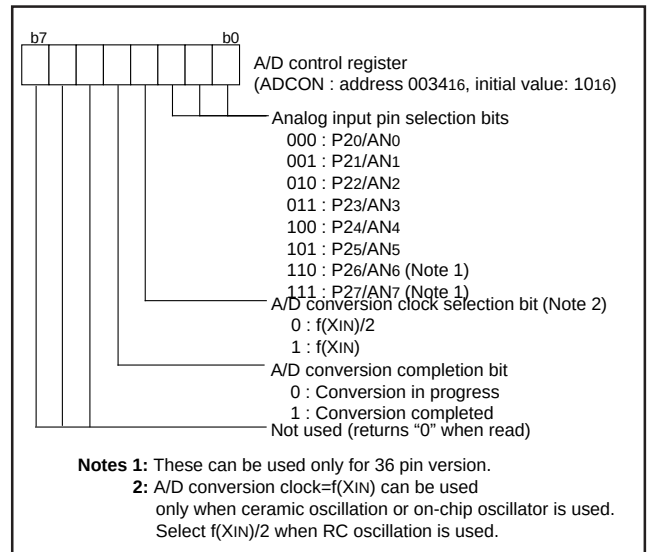
Fig. 65 Structure of A/D control register
