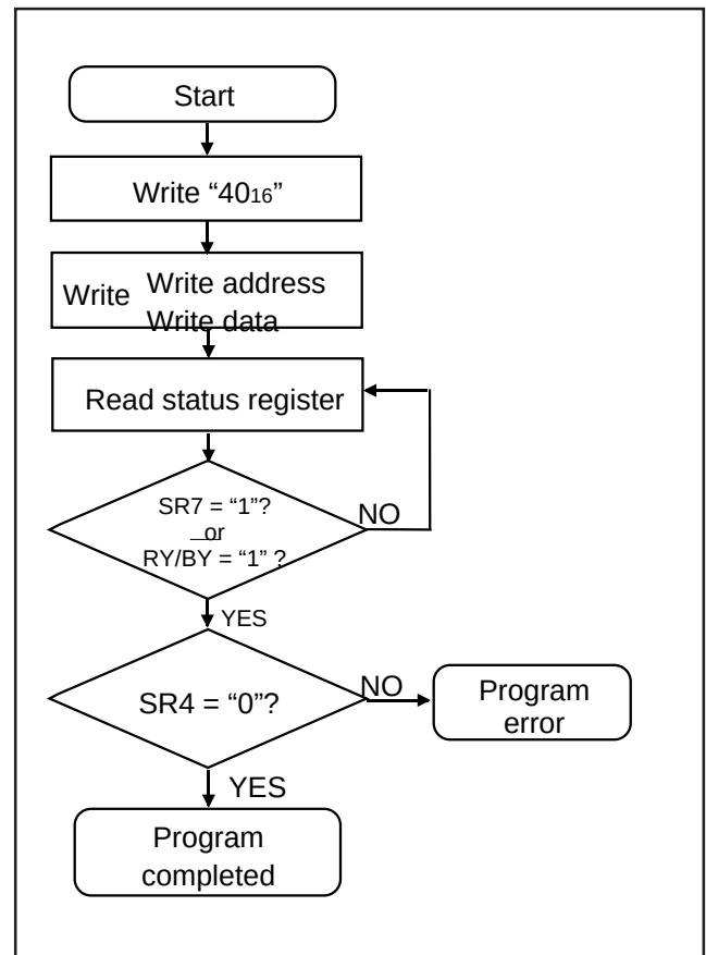
Fig. 99 Program flowchart
