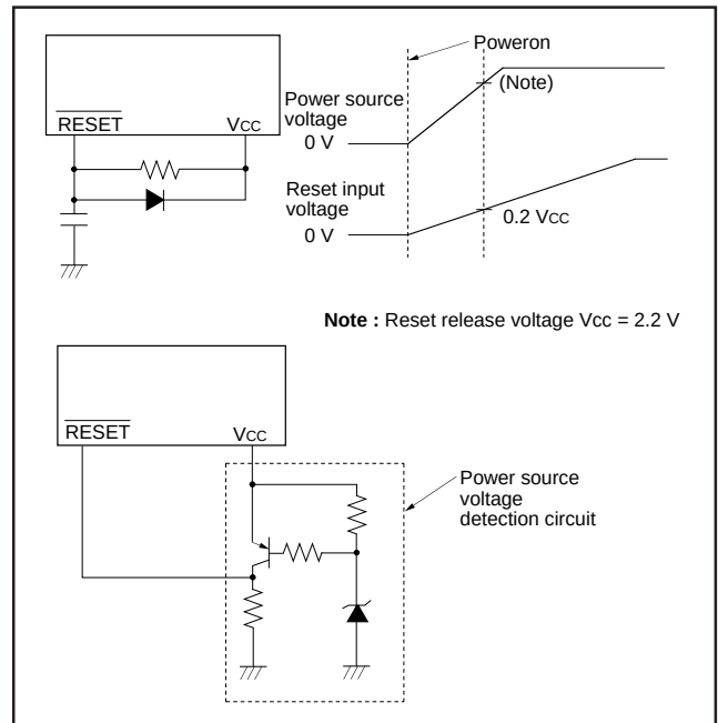
Fig. 70 Example of reset circuit
