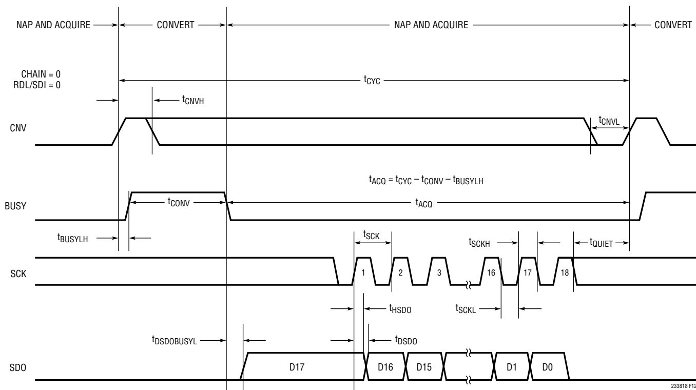
Figure 12. Using a Single LTC2338-18 in Normal Mode
