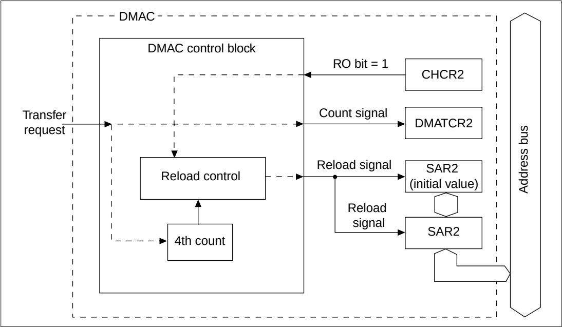
Figure 11.25 Source Address Reload Function
