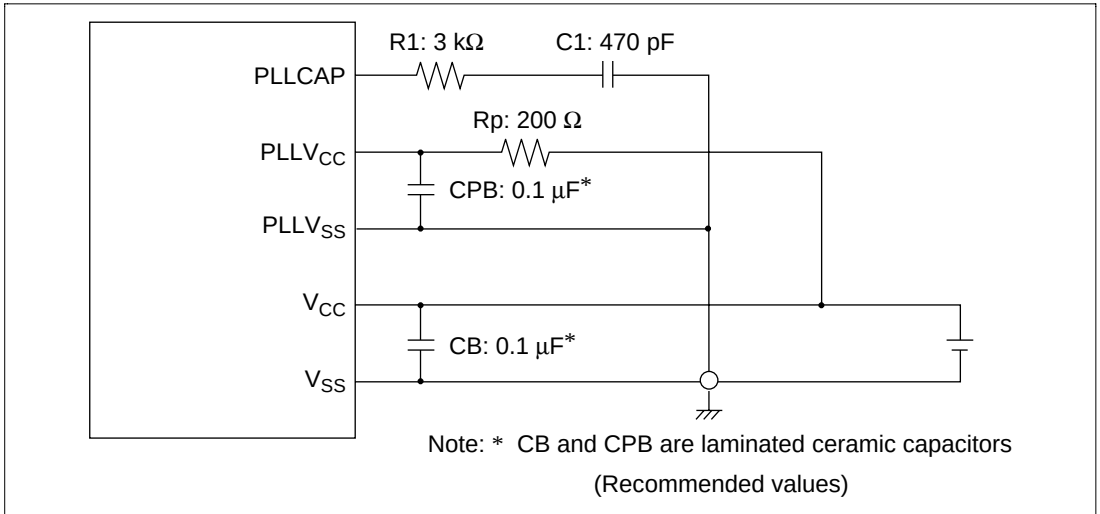
Figure 4.6 Cautions for Use of PLL Oscillator Circuit
