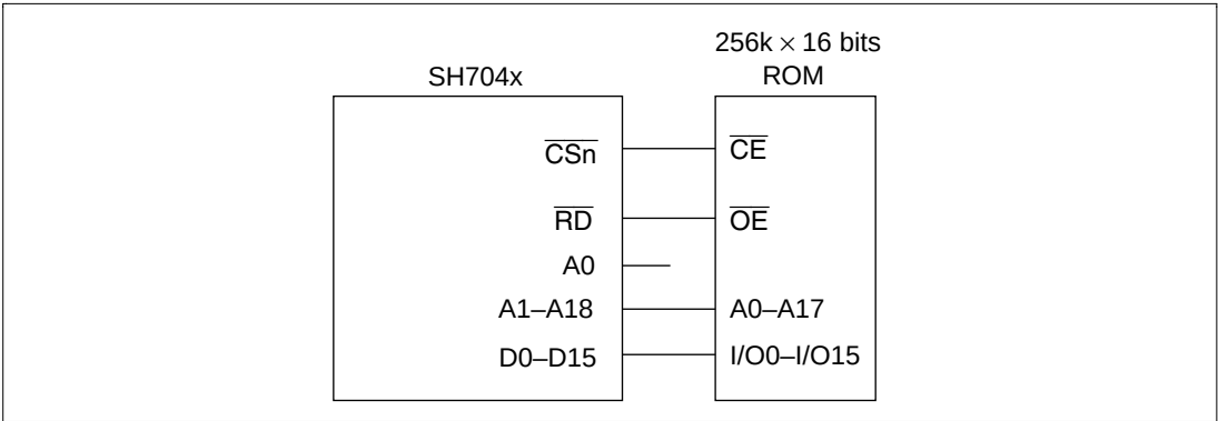
Figure 10.24 16-Bit Data Bus Width ROM Connection
