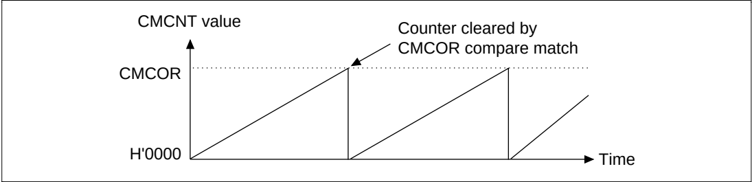
Figure 17.2 Counter Operation
