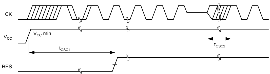
Figure 26.3 Oscillation Settling Time
