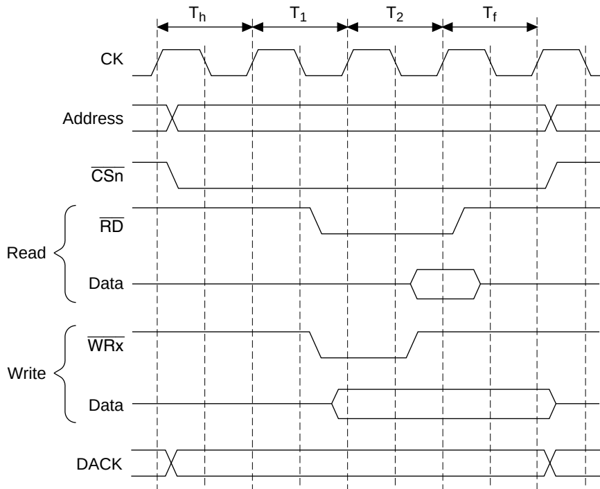
Figure 10.6 \overline{\text{CS}} Assert Period Extension Function
