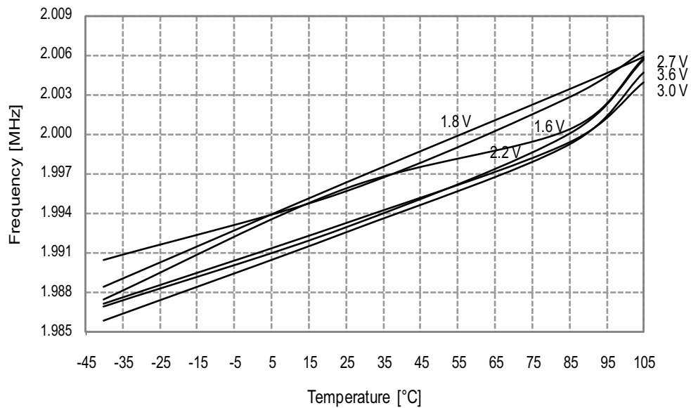
Figure 33-129. 2MHz Internal Oscillator Frequency vs. Temperature DPLL enabled, from the 32.768kHz internal oscillator
