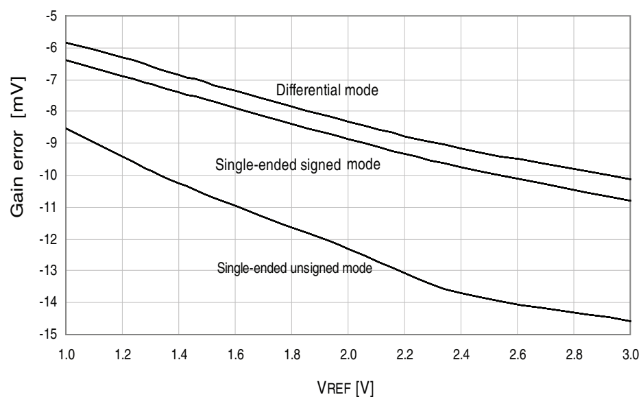
Figure 33-178. Gain Error vs. V_{REF}
