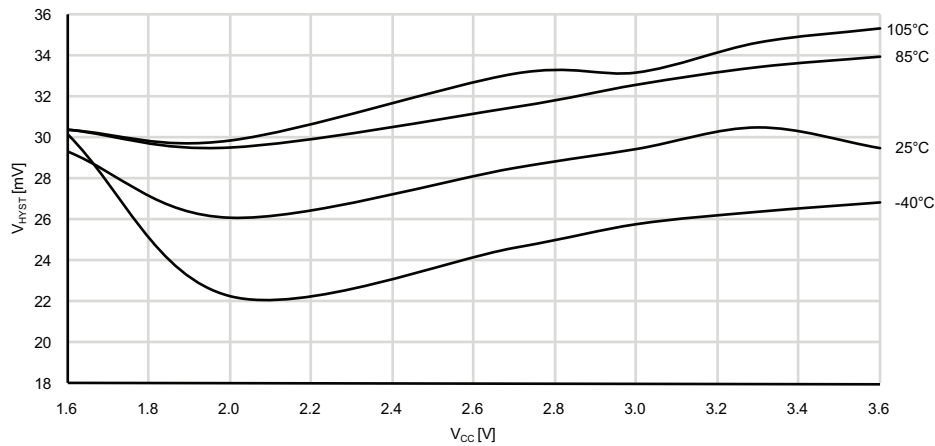
Figure 33-324. Analog Comparator Hysteresis vs. V_{CC} Large hysteresis high speed mode; large hysteresis
