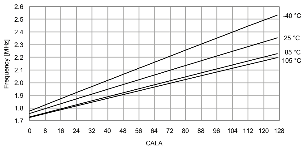
Figure 33-270. 2MHz Internal Oscillator Frequency vs. CALA Calibration Value V_{CC} = 3V
