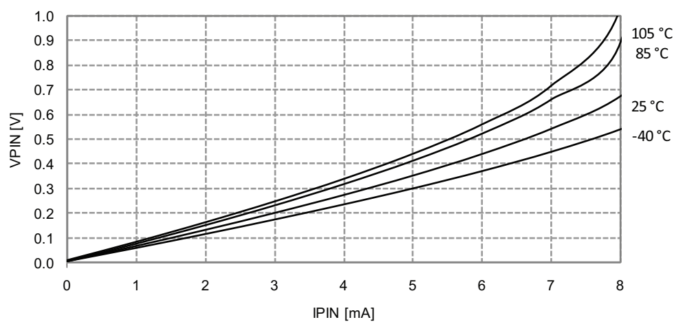
Figure 33-236. I/O Pin Output Voltage vs. Sink Current
