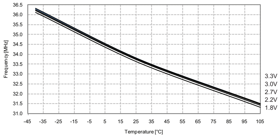
Figure 33-341. 32MHz Internal Oscillator Frequency vs. Temperature DFLL disabled
