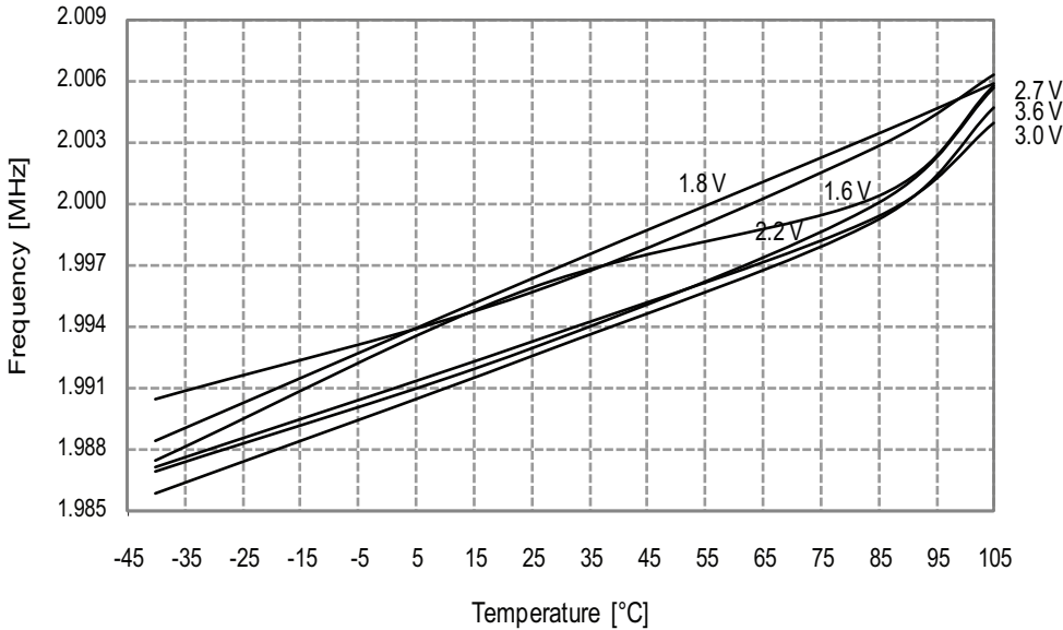
Figure 33-58. 2MHz Internal Oscillator Frequency vs. Temperature DFLL enabled, from the 32.768kHz internal oscillator
