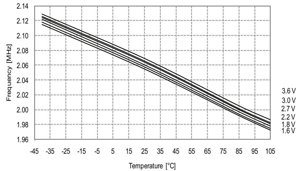
Figure 33-58. 2MHz Internal Oscillator Frequency vs. Temperature DFLL enabled, from the 32.768kHz internal oscillator
