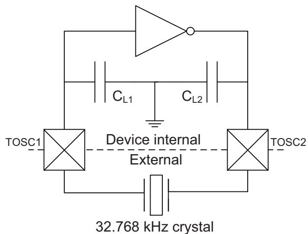
Figure 32-25. TOSC Input Capacitance
