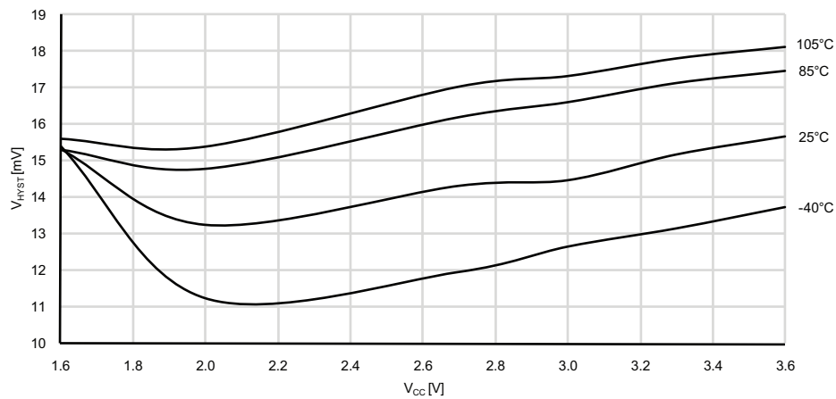
Figure 33-323. Analog Comparator Hysteresis vs. V_{CC} Small hysteresis high speed mode; small hysteresis
