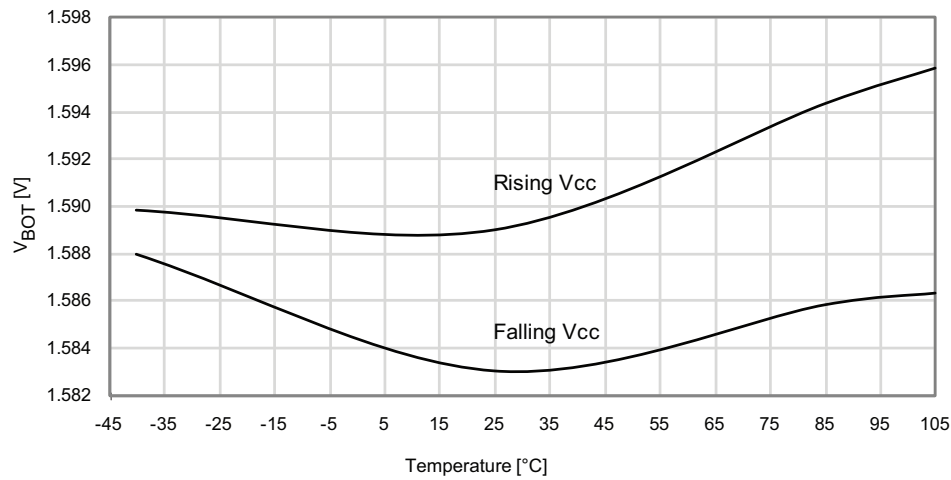
Figure 33-188. BOD Thresholds vs. Temperature BOD level = 1.6V
