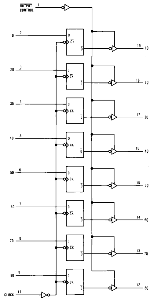
Logic Diagram
