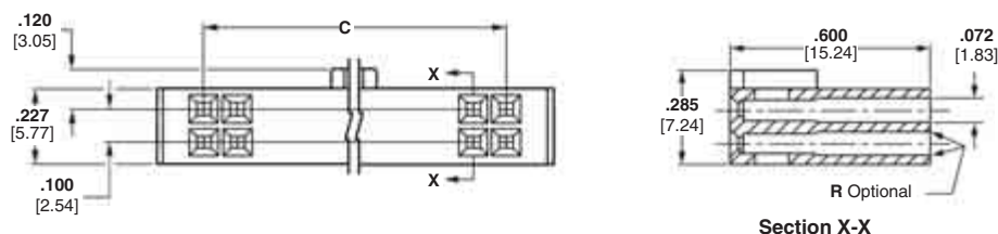
Section X-X
