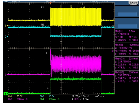
FIGURE 9. LX, VIN, IL AND IO AT PWM DIMMING
