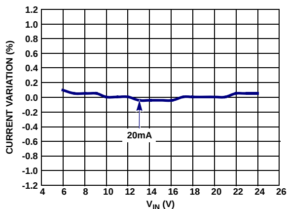
FIGURE 5. CURRENT REGULATION
