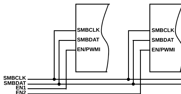
FIGURE 31. MULTIPLE DRIVERS OPERATION
