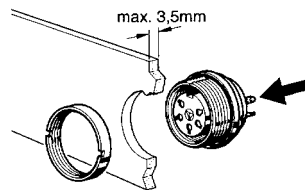
Assembling instruction
