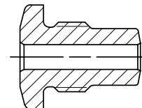
124449 DRIVING ANVIL -06
