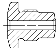
124450 DRIVING ANVIL -05
