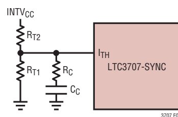
Figure 8. Active Voltage Positioning Applied to the LTC3707-SYNC
