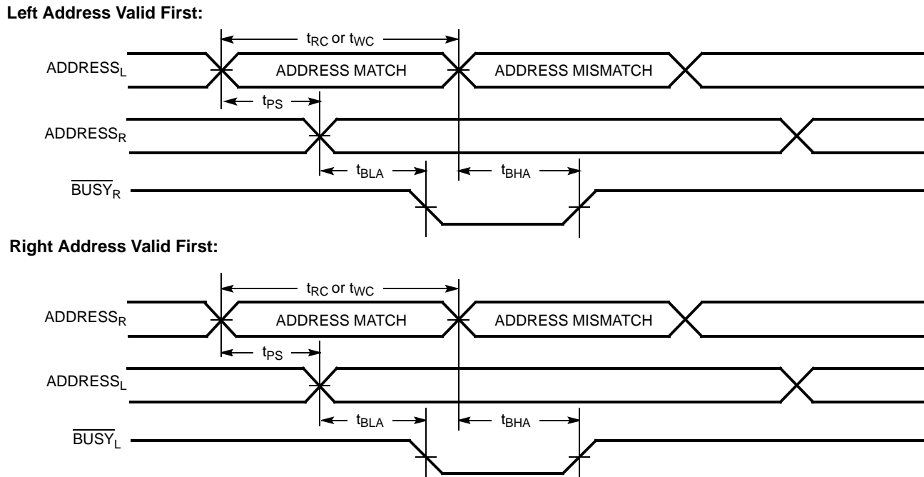
Figure 13. Busy Timing Diagram No. 2 (Address Arbitration) [37]
