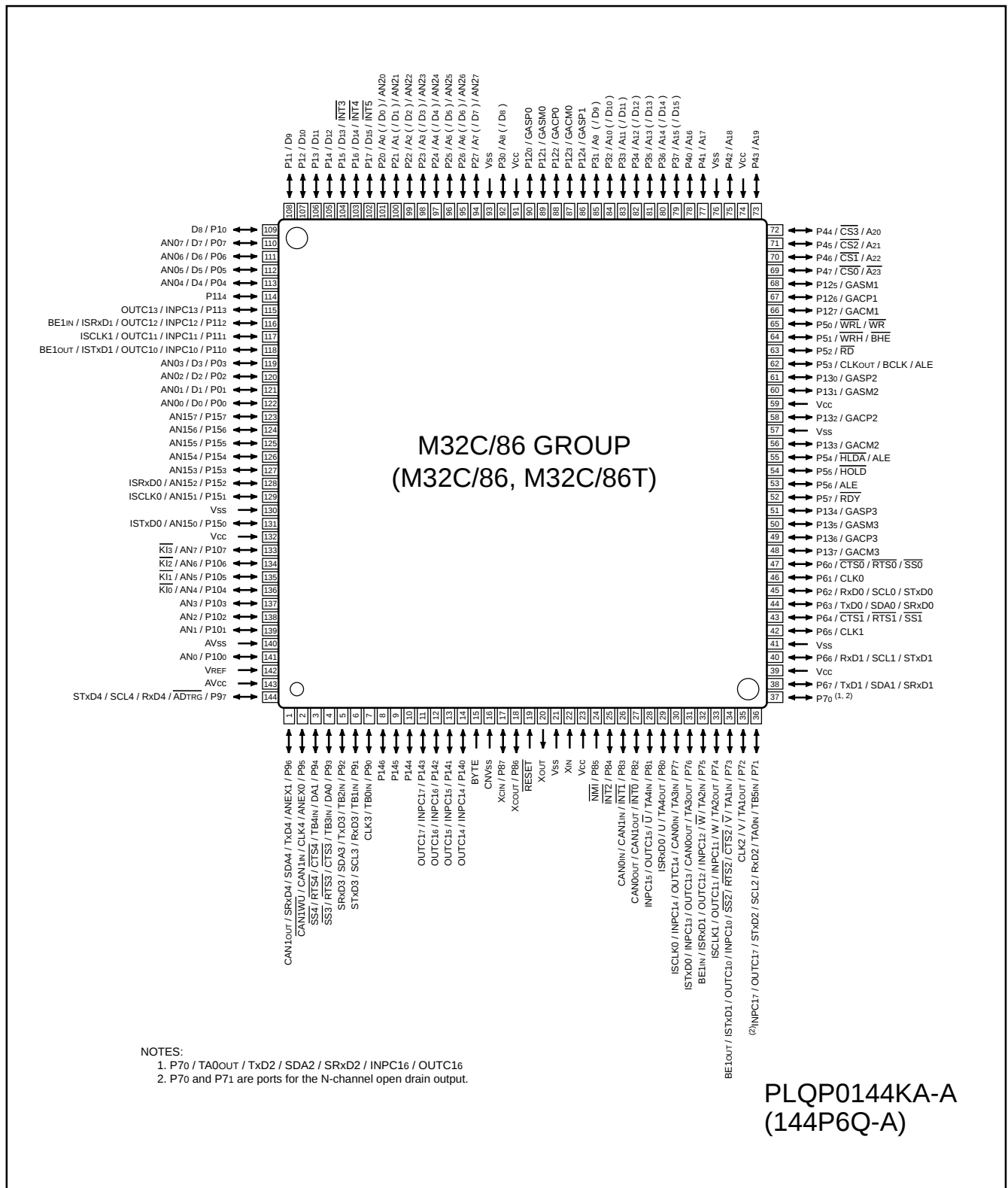
Figure 1.3 Pin Assignment
